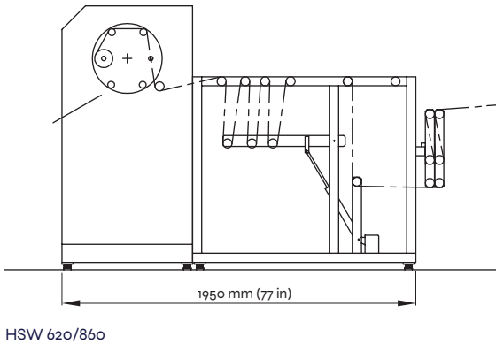
HSW Winder
