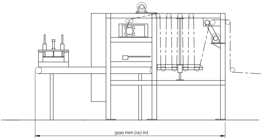
FW Winder
